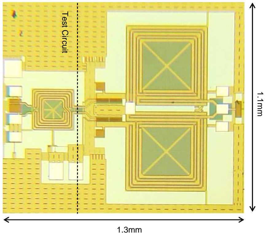
Figure 4.14: Die microphoto for the one-stage PA.
