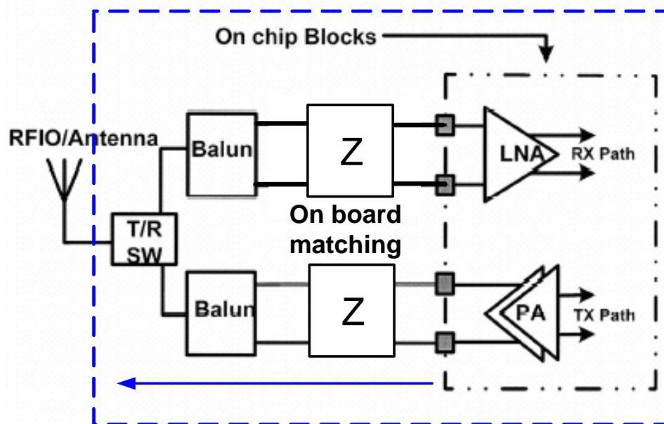
Figure 1.2: Conventional RF front-end architecture.
