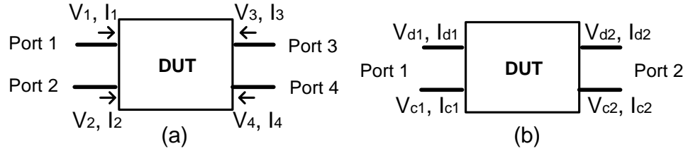
Figure 2.3: A 4-port device: (a) single-ended: ports referenced to ground; (b) mixed-mode: ports are in pairs, both with differential mode and common mode.
