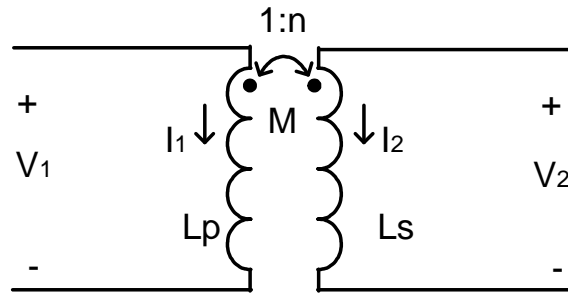
Figure 2.1: An ideal transformer.
