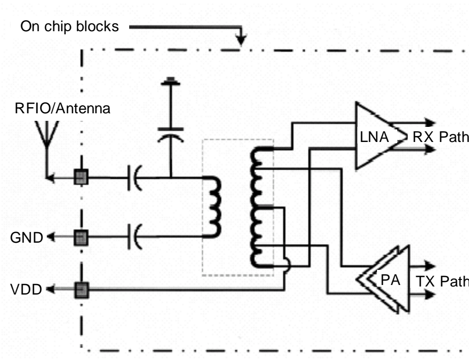
Figure 1.3: Transformer-based balun solution for Bluetooth applications.
