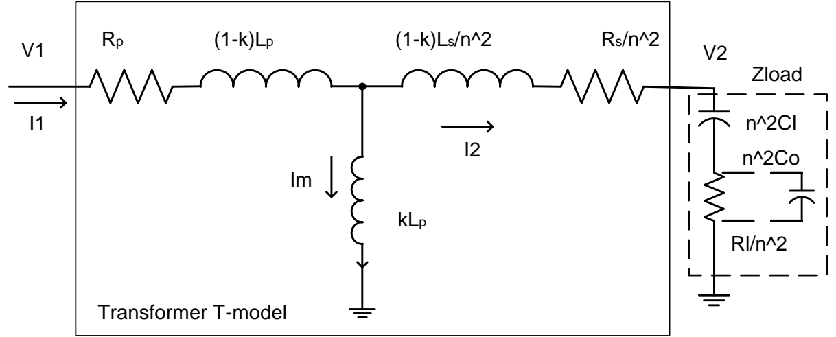
Figure 2.16: Transformer equivalent T-model with load impedance.
