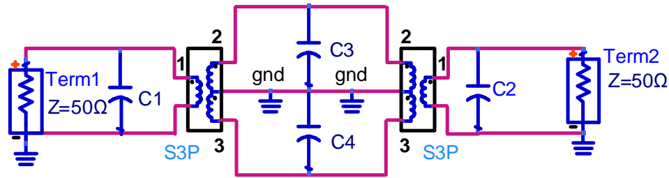
Figure 4.10: Back-to-back simulation setup to get minimum insertion loss.
