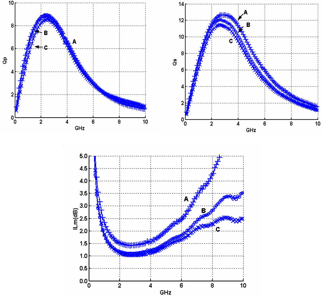
Figure 3.9: Q_p , Q_s and IIm comparison for transformers with same D_{out} = 400 \mu\text{m} .
