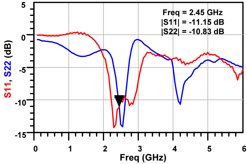
Figure 4.15: S_{11} and S_{22} of the PA.
