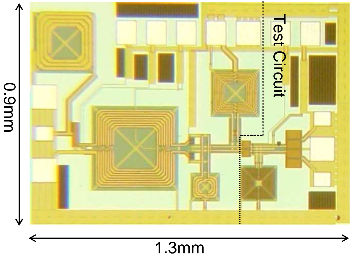
Figure 5.6: The die microphoto for the receive path.
