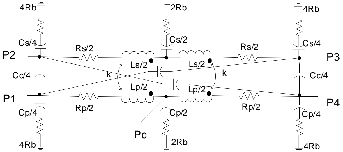
Figure 2.7: Transformer frequency dependent circuit model.
